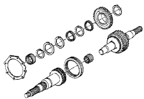
T350-400 Gear Train
