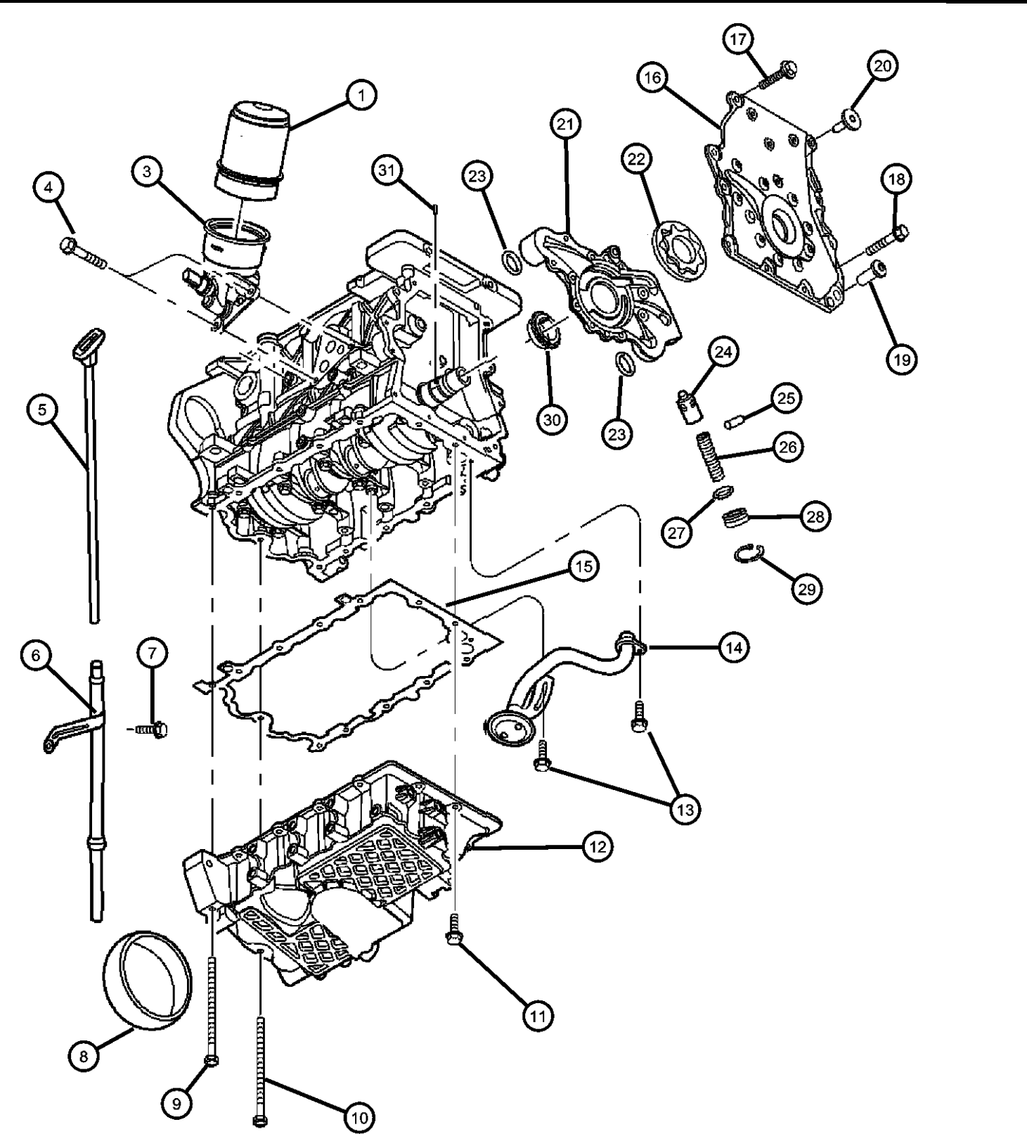
Engine, Oiling [EJD] Figure 1.6L-710
